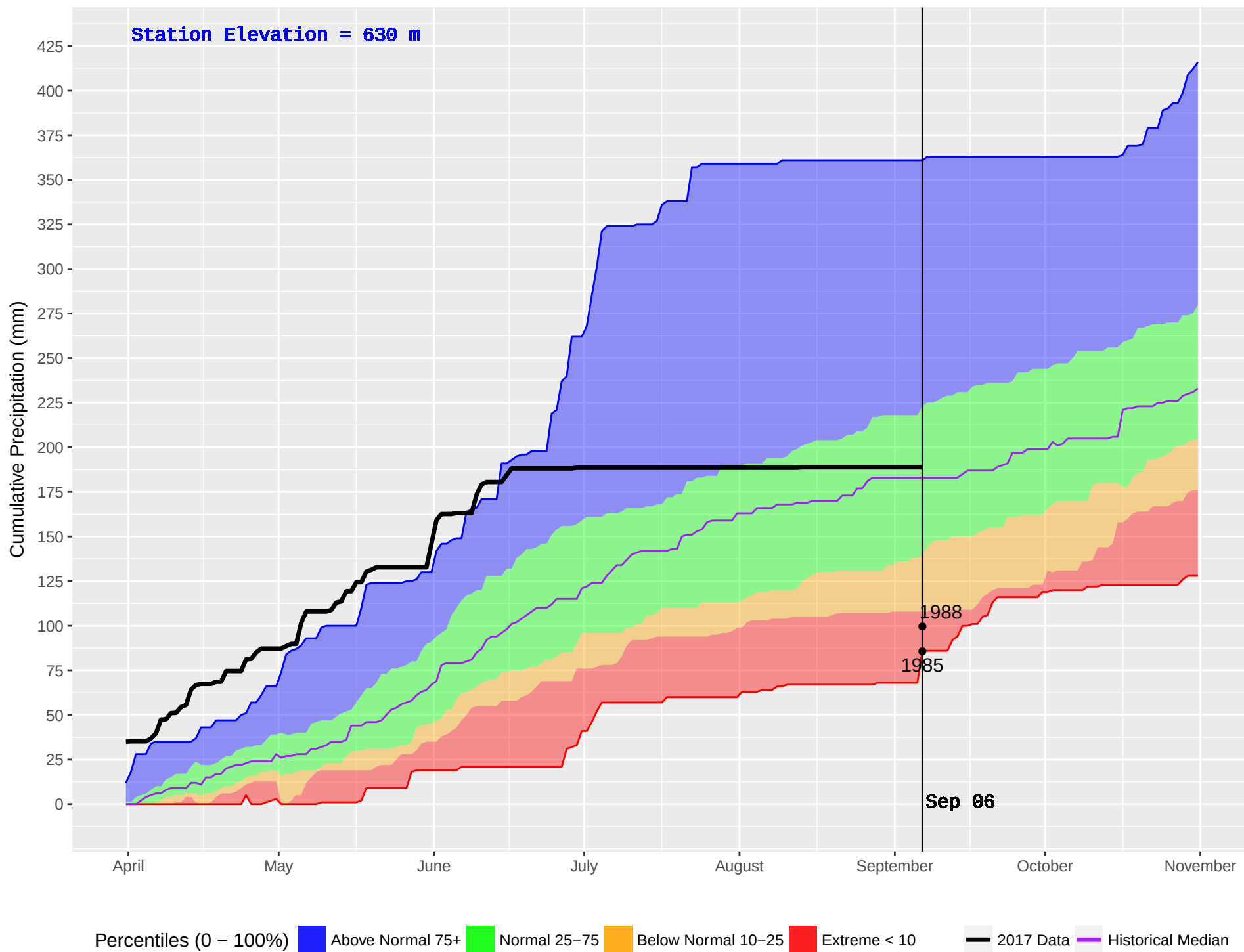
GRAND FORKS (392) : Historical (1981–2016) and Current (2017) Noon Cumulative Precipitation
